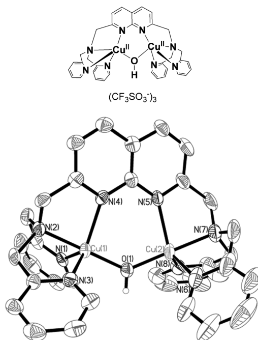
Figure 1. Top: The structure of the dicopper(II) catalyst, [\text{Cu}_2(\text{BPMAN})(\mu\text{-OH})]^{3+}(\text{OTf})_3 . Bottom: ORTEP view (thermal ellipsoids set at 50% probability) of the cation of [\text{Cu}_2(\text{BPMAN})(\mu\text{-OH})]^{3+} . The counterions and hydrogen atoms are omitted for clarity. Selected bond lengths [Å] and angles [°]: Cu(1)–O(1) 1.883(4), Cu(1)–N(1) 2.062(5), Cu(1)–N(2) 2.009(5), Cu(1)–N(3) 2.099(5), Cu(1)–N(4) 2.200(5), Cu(2)–O(1) 1.864(4), Cu(2)–N(5) 2.201(5), Cu(2)–N(6) 2.073(7), Cu(2)–N(7) 2.004(6), Cu(2)–N(8) 2.085(6); Cu1–O1–Cu2 131.7(2).
